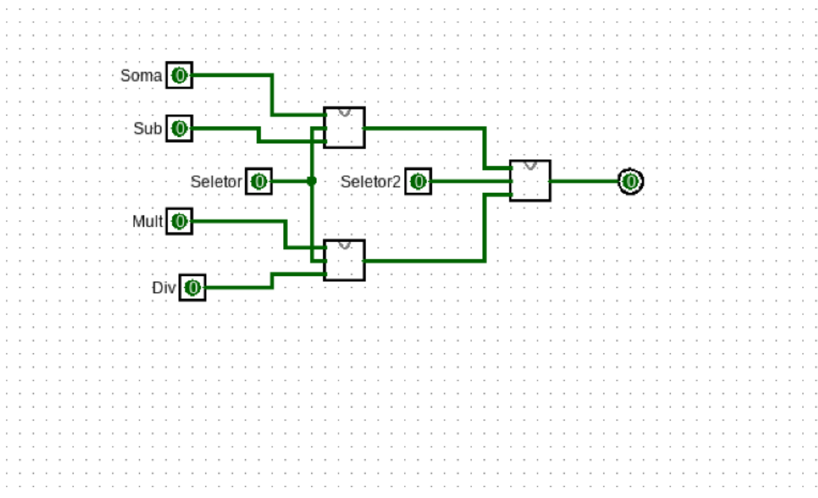
Mux 4-1
